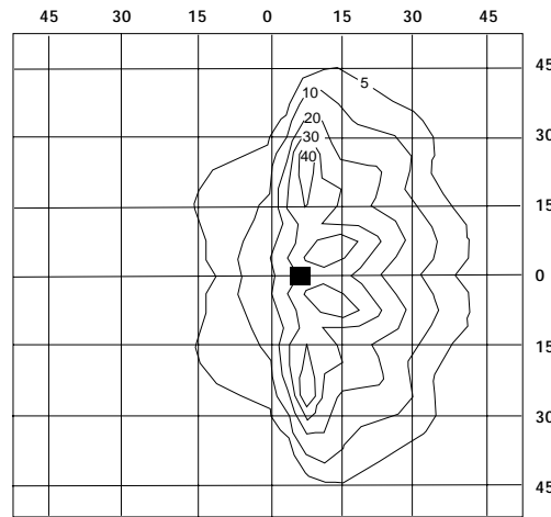
Single Fixture - 1000W MH Initial Lumens At 25' Mounting Height
