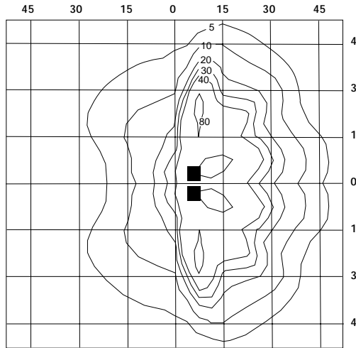
Double Fixture - 1000W MH Initial Lumens At 25' Mounting Height
